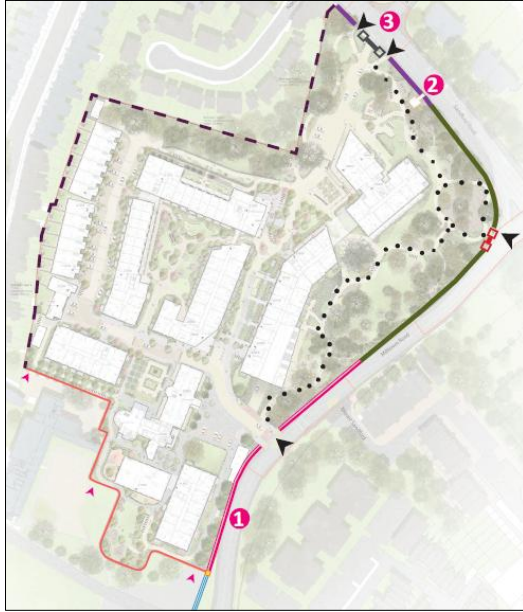
Figure 4.12: Boundary Treatment Strategy Fronting Sanford Road and Milltown Road Now Proposed
