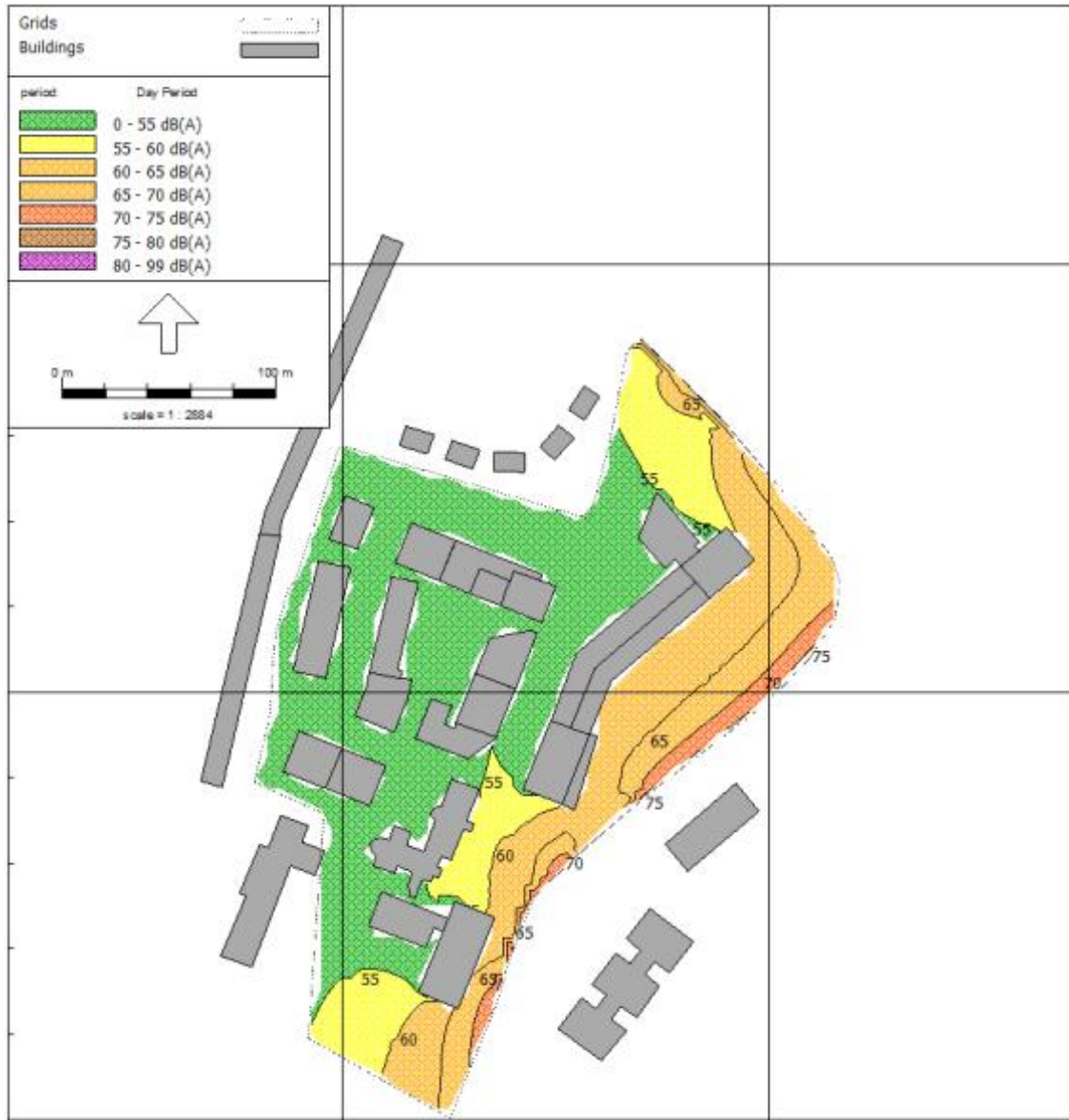
Figure 13.14: Predicted Noise Levels across External Areas (1.5m above ground)
